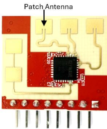
Front view (antenna facing forward)
